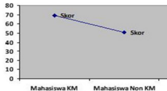
Fig. 1: Average Score of Student Social Skills
